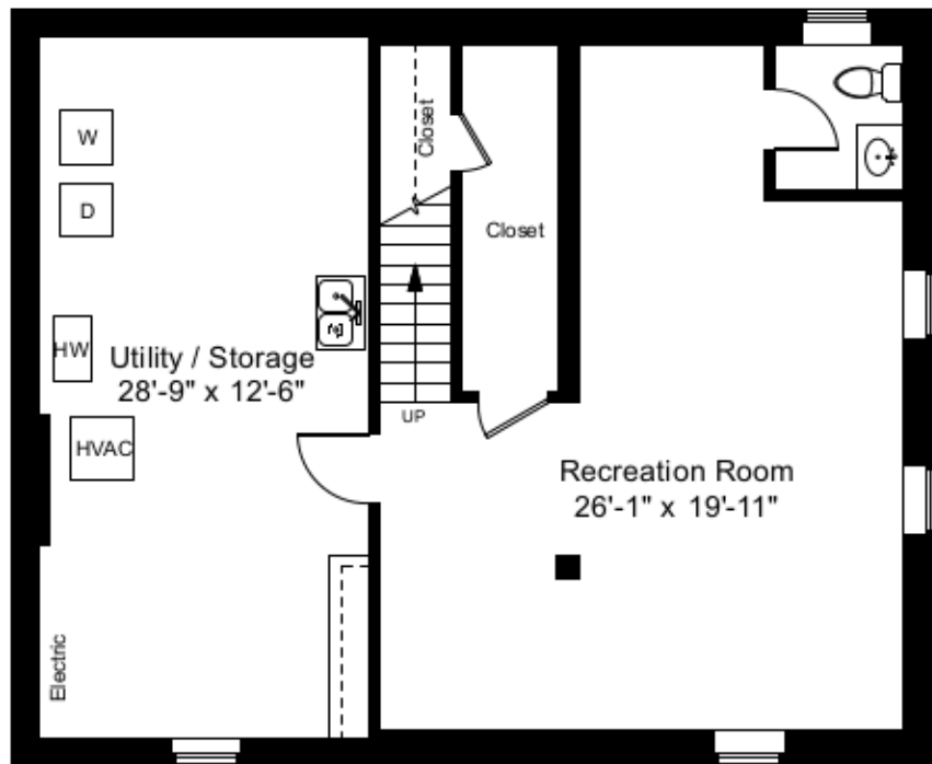
Lower Level Plan Ceiling Height = 6'-9"
