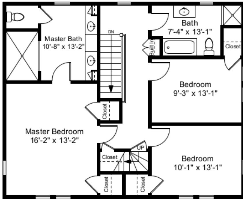
Second Floor Plan Ceiling Height = 8'-8"
