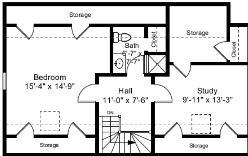
Third Floor Plan Ceiling Height = 7'-0"
